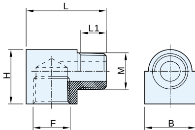
ELBOW C
